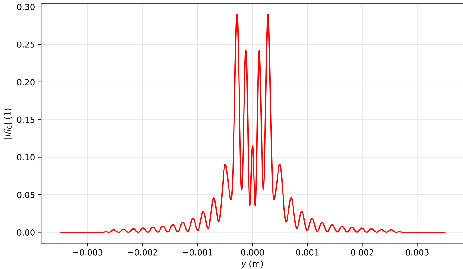
Intensity profile I(x=0, y, z=0.159)/I_0 , \text{Pin}=7.0\text{Pcr} , artificial time
